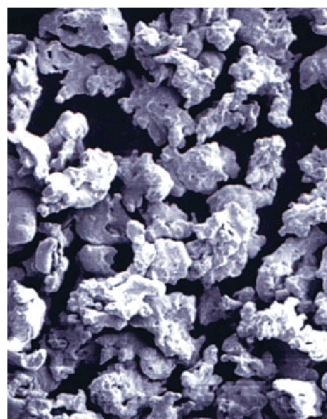
P316L STAINLESS STEEL POWDER
